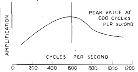
FIG. 2 This is a curve of a typical A.F. transformer, showing the limited efficiency range.
