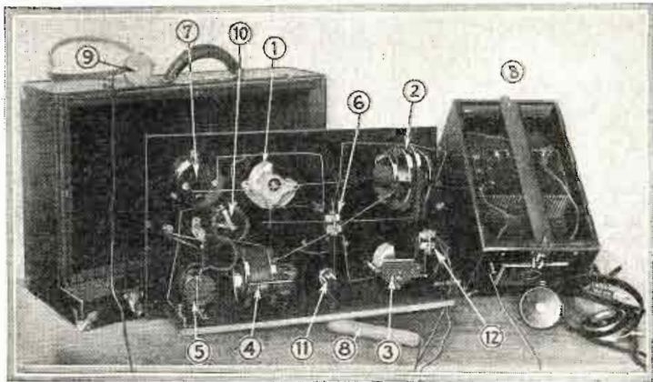
The interior of the Kiro-Vox. 1 and 3 are variable condensers; 2, a variometer; 4, variocoupler; 5, a head-phone; 6 and 12, fixed condensers; 7, voltmeter; 8, search electrode; 9, head electrode; 10, rheostat; 11, battery switch, and B, the battery cabinet.
