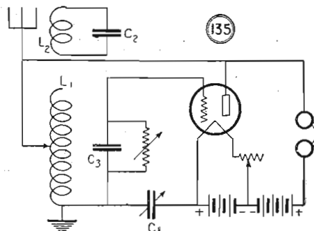
The variation of the ultra-audion circuit shown above will prove to be popular with one's neighbors, as it will not radiate.
