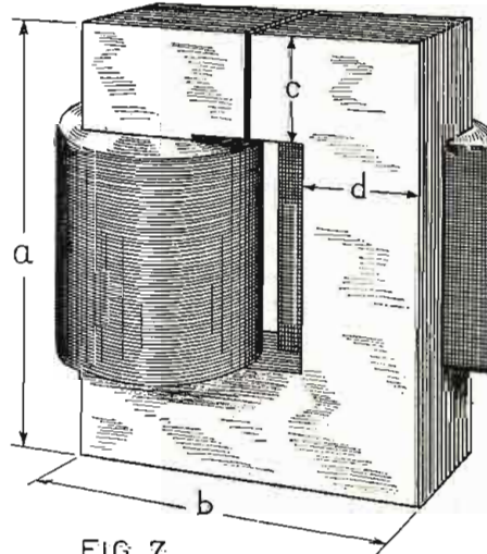
FIG. 7 Dimensions are given in the accompanying table for two different sizes of choke coils; one for receiving and the other for transmitting purposes.
