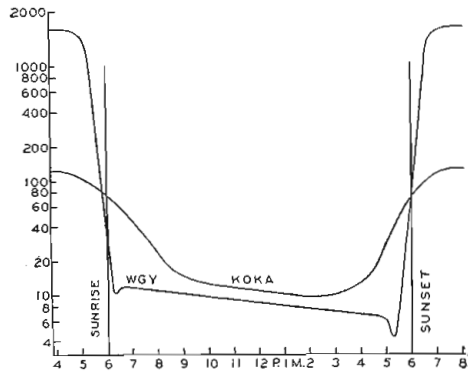
The above audibility chart shows plainly the drop in signal strength with the sunlight and its rise again at sun down.
