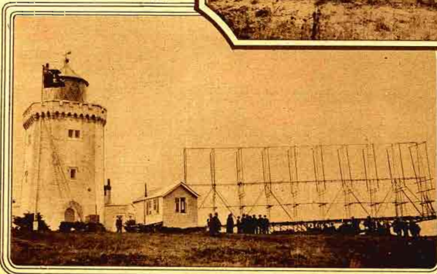
TRACK FOR THE REVOLVING ANTENNA. As the antenna must transmit signals to every point of the compass, the circular track, shown in the photograph on the right, is necessary. The details of the construction can be easily seen. Photos by Wide World.
