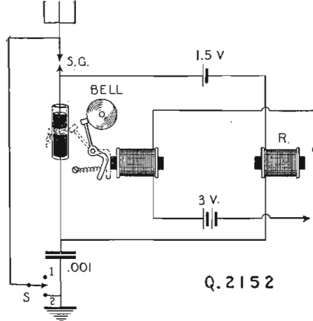
Q. 2152 A "storm detector." The coherer operates in a horizontal position. The metal plugs are preferably slanted, rather than straight-faced as shown.
