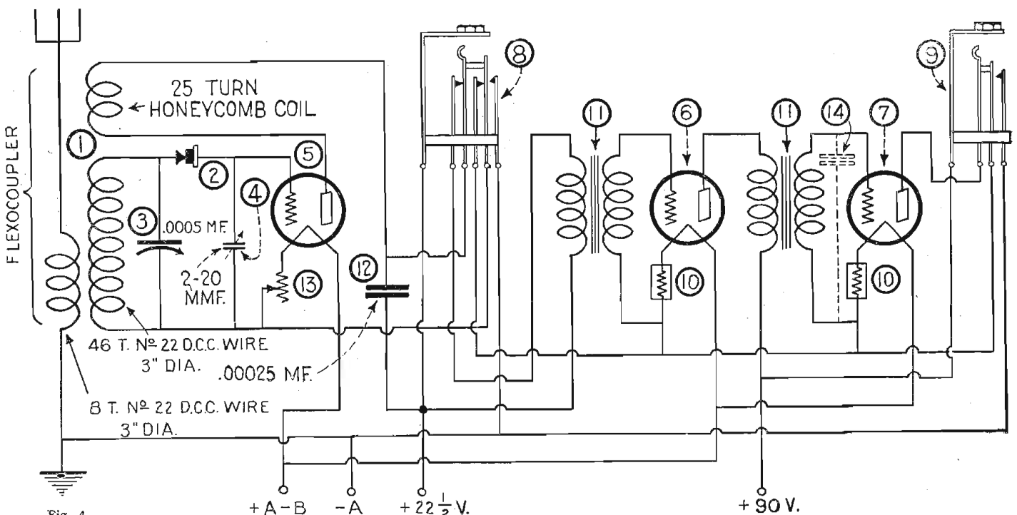
Fig. 4 Complete circuit diagram of 3-tube Regenerative Interflex Circuit. (1) is the Flexo-Coupler, (2) crystal detector, (3) variable condenser, (4) Small balancing condenser, (5) detector-coupled audio amplifier tube, (6) second audio tube, (7) third audio tube, (8) and (9) filament control jacks, (10) Amperites, (11) audio transformers, (12) fixed condenser, (13) carbon type rheostat.
