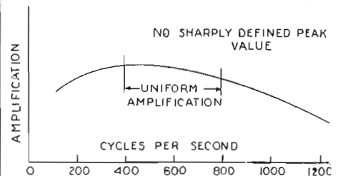
FIG. 3 In the best transformers, the amplification curve is rather uniform between certain frequencies, but not over the entire range.
