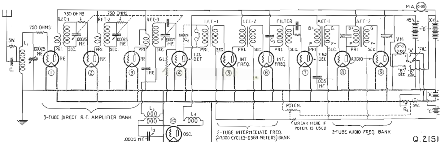
The Experimenters' Information Service Navy Model C-10 super-heterodyne designed for a wave-length range from 600 meters down to 50 meters, the band being covered through the expedient of interchangeable coils. Blueprints are not available.
